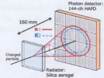
Figure 1: The principle of the particle identification with the ARICH counter
