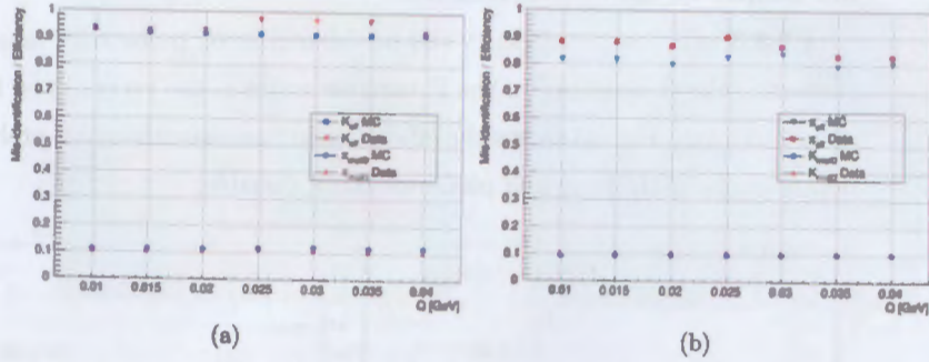
Figure 14: Kaon and pion efficiency and mis-identification probability dependence over Q variable.
