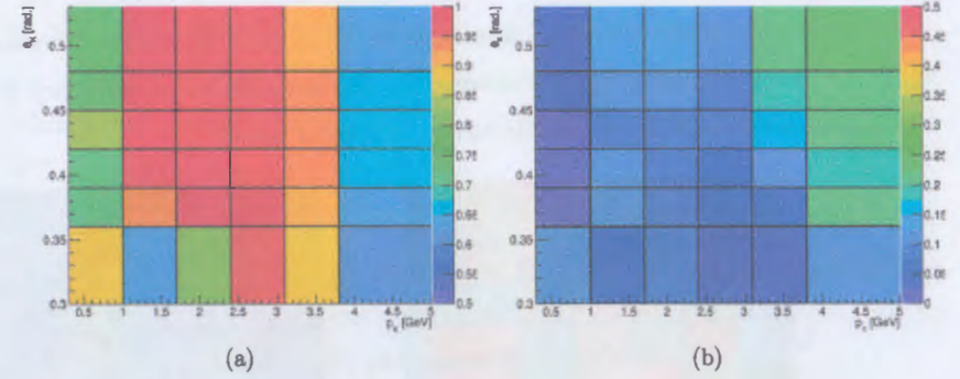
Figure 9: 2D efficiency plot for kaon(a) and mis-identification plot(b) for pion based on Data results.
