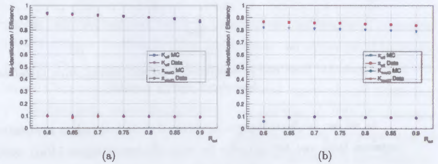
Figure 13: Koan and pion efficiency and mis-identification probability dependence over R variable.
